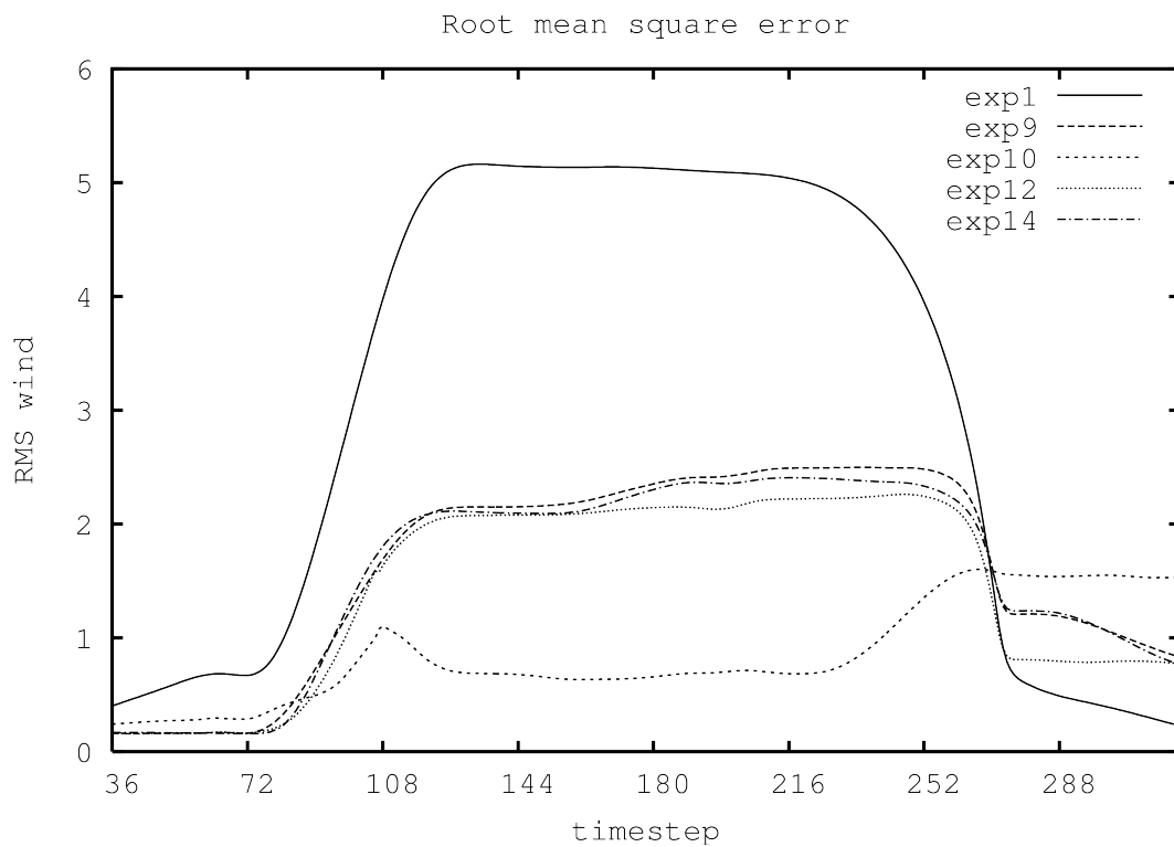
Figure 4.13: Root mean square error of wind variable (m/s) computed over the LAM domain using the LAM coupled to low resolution global model for each time step as reference, for LAM coupled using flow relaxation scheme to low resolution global data with 3 h interval interpolated linearly in time (exp1, full line), coupled in gridpoint space but the large scale data are interpolated in spectral space: when the amplitude and phase of the spectral components are interpolated in time using amplitude (exp9, long dash) extrapolation (exp10, short dash), integration between coupling steps (exp12, dots) or polynomial interpolation in time (exp14, dot dash).
