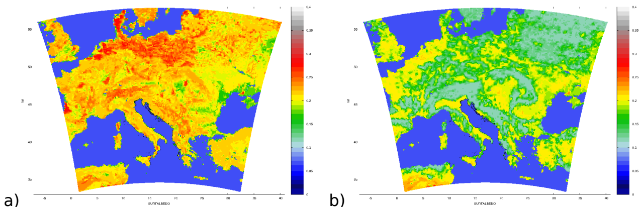
Figure 14. Input surface albedo (a) and output (b) when the vegetation albedo is included into the total albedo.
