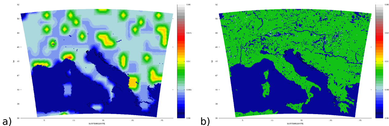
Figure 9. Surface emissivity in the clim file (a) and computed using the land sea mask data from the SURFEX PGD file (b).
