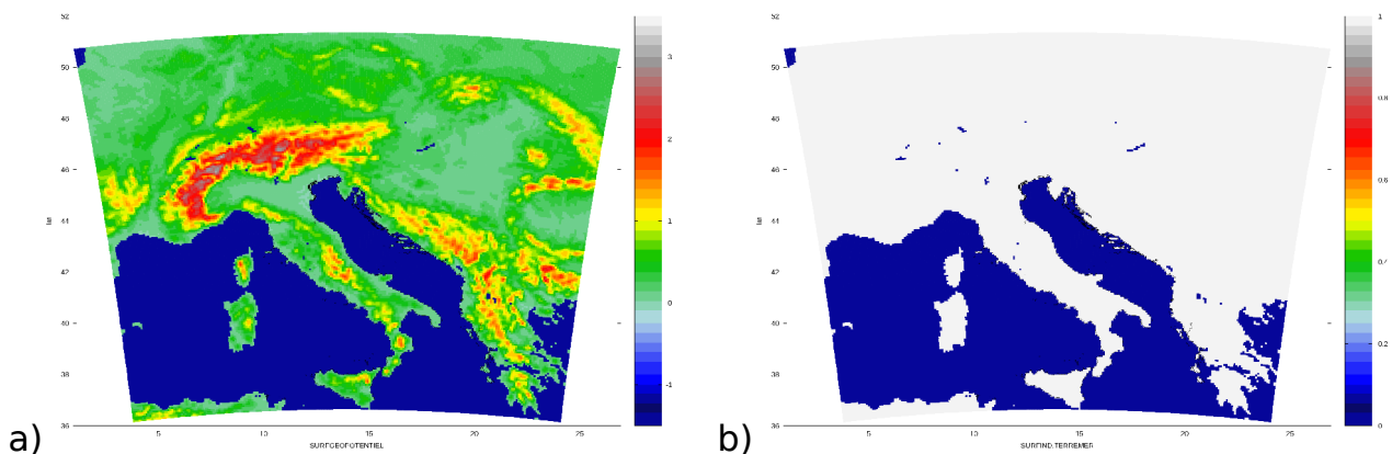
Figure 1. Surface geopotential (a) (divided by 9.81 and 1000 to represent terrain height in km and forced to -1 above the sea) and land sea mask (b) with LNORO, and LNLISM true for the domain in 8 km resolution.
