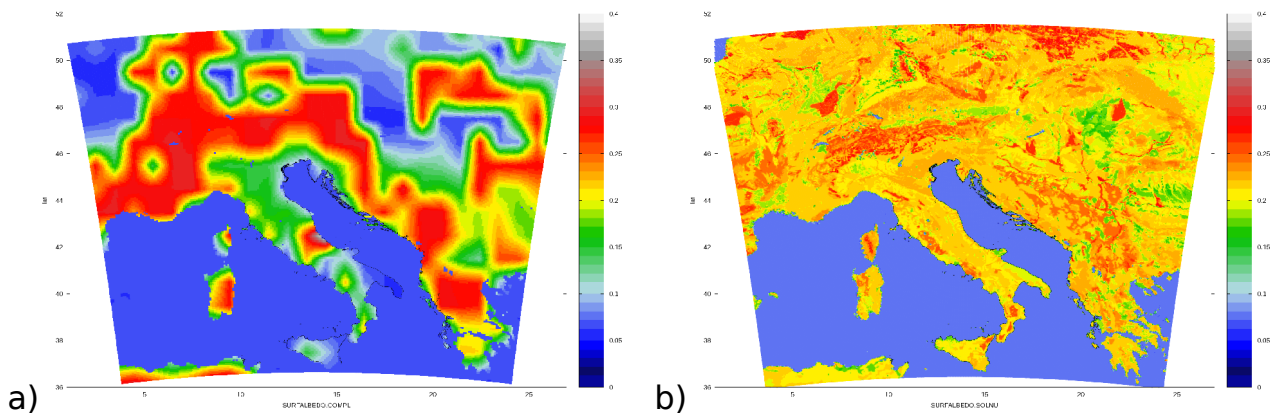
Figure 8. Albedo of bare ground in the clim file (a) and computed using the soil type data from the SURFEX PGD file (b).
