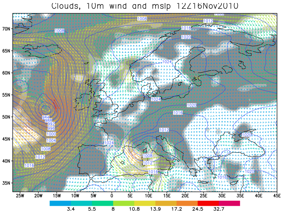
Figure 5. ERA Interim 10 m wind (colour of the vectors shows wind speed in m/s as on the colour bar below), mean sea level pressure (blue isolines) and cloudiness (shades of gray) for 12 UTC on 16 November 2010.
