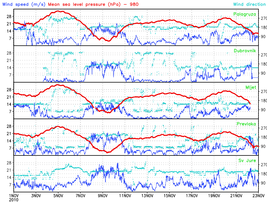
Figure 6. Measured wind speed (dark blue, scale on the left) and mean sea level pressure (red) reduced by 980 hPa (to fit the scale on the left) and wind direction (light blue, in degrees from north clockwise, scale on the right) for November 2010. Sv. Jure is marked as Biokovo in Fig. 1.
