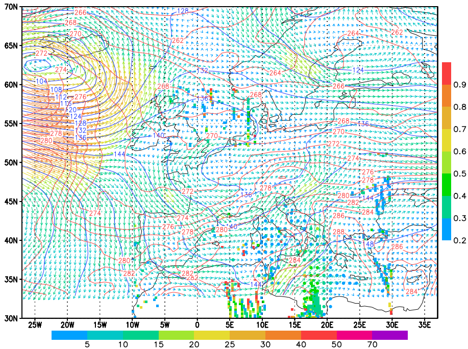
Figure 3. ERA Interim 850 hPa wind (colour of the vectors shows wind speed in m/s as on the colour bar below), geopotential (blue isolines) and temperature (red isolines) with measured aerosol optical thickness at 12:00 UTC 7 November 2010 from MODIS (circles) and OMI (squares). AOT is shown in colour according to the colour bar on the right.
